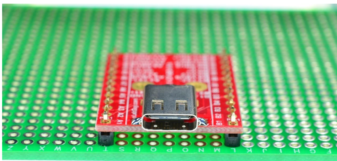
Figure 5: Solid Mounting on prototype PCB
