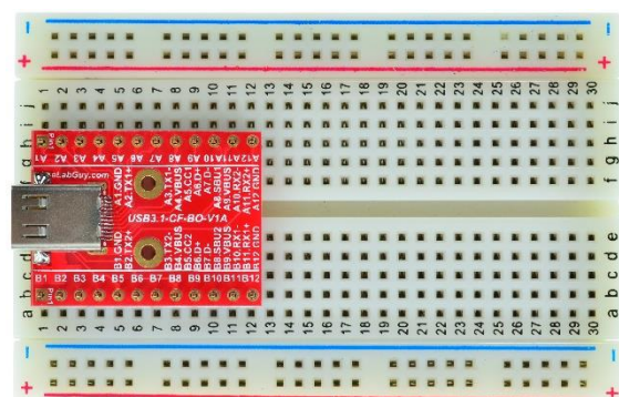
Figure 2: Example of connecting the USB3.1-CF-BO-V1A on a breadboard
